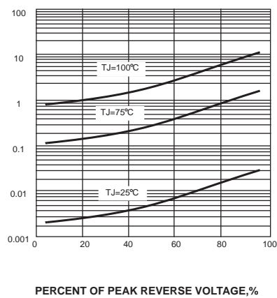
FIG. 4-TYPICAL REVERSE CHARACTERISTICS
